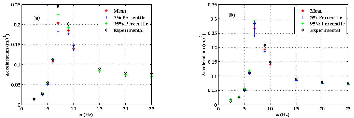
Figure 6: Uncertainty propagation: acceleration response spectra uncertainty along with comparisons with the experimental data for the suspension component. (a) moderate excitation level, (b) strong excitation level.
