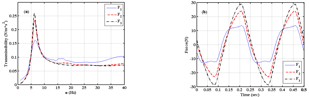
Figure 3: (a) Transmissibility function of the support system, for three different forcing levels, (b) History of the external force applied with a fundamental harmonic frequency \omega = 4\text{Hz}
