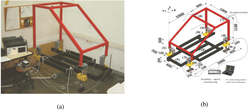
Figure 1: (a) Experimental set up of the structure tested, (b) Dimensions of the frame substructure and measurement points.
