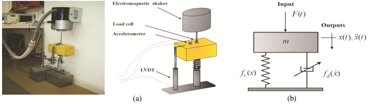
Figure 2: (a) Experimental set up for measuring the support stiffness and damping parameters, (b) Equivalent model.
