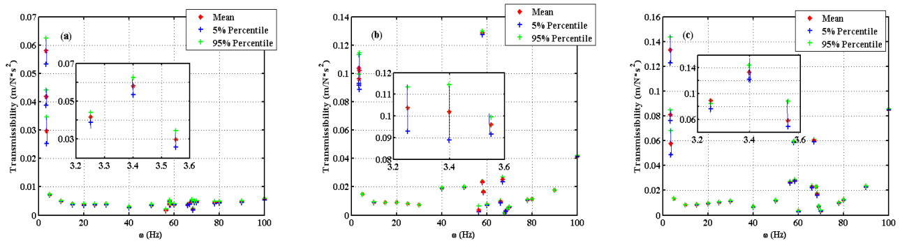
Figure 7: Uncertainty propagation: acceleration transmissibility function uncertainty for combined system. (a) wheel DOF, (b) DOF at connection between suspension and frame, (c) frame DOF.
