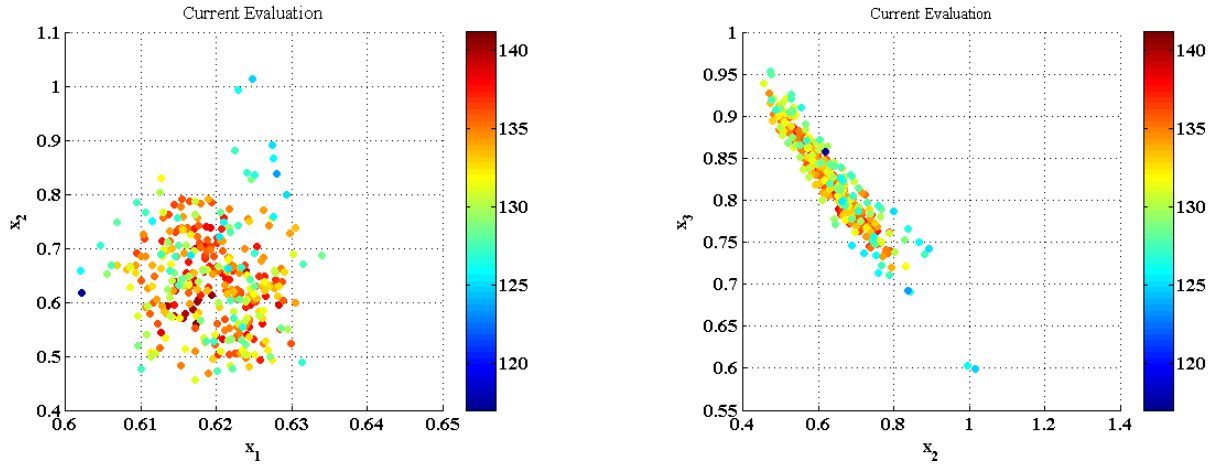
Figure 4: Model parameter uncertainty: projection of TCMC samples in the two dimensional parameter spaces
