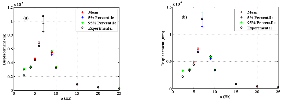
Figure 5: Uncertainty propagation: displacement response spectra uncertainty along with comparisons with the experimental data for the suspension component. (a) moderate excitation level, (b) strong excitation level
