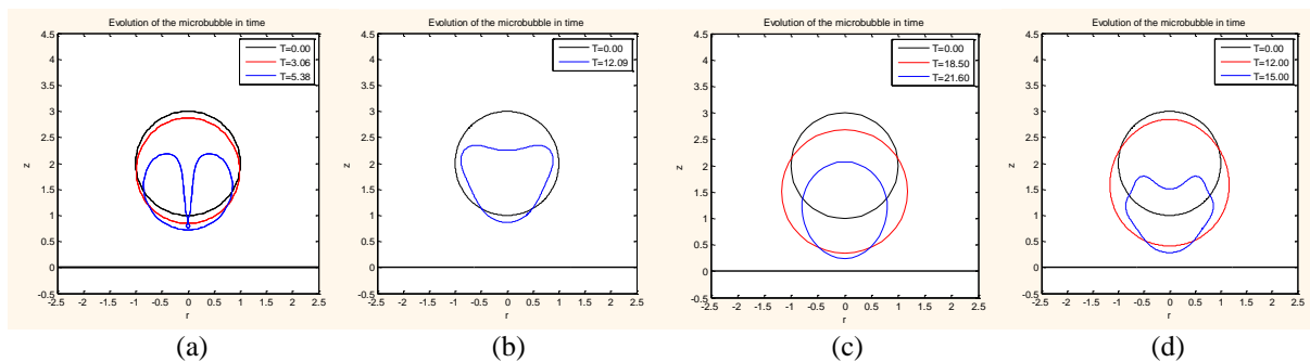
Figure 1: (a) Shape sequence of a free bubble and (b) a coated microbubble approaching a rigid wall, subject to a step pressure change. Shape sequence of a coated microbubble approaching a rigid wall, subject to a sinusoidal pressure change for (c) a relatively small ( \varepsilon=2 ) and (d) a large amplitude ( \varepsilon=3 ) of the acoustic disturbance; simulation parameters are set to: R_0=3.6 \mu\text{m} , G_s=80 \cdot 10^6 , \mu_s=20 \text{ Pa}\cdot\text{s} , k_B=3 \cdot 10^{-14} \text{ N}\cdot\text{m} , b=0 (Mooney-Rivlin shell), \nu_0=1 \text{ MHz} , \nu_i=1.7 \text{ MHz} , \gamma=1.07 , P_{st}=101325 \text{ Pa} , \delta=1 \text{ nm} .
